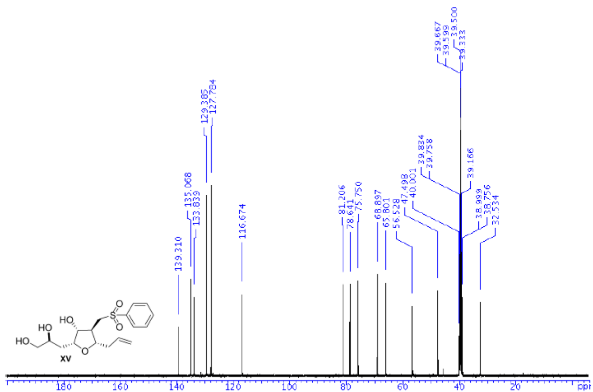
Figure S4 ^{13}\text{C} NMR of compound XV
