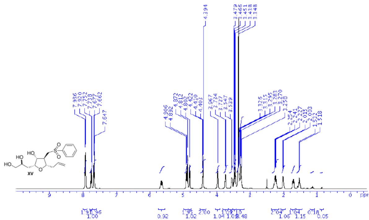
Figure S3 ^1\text{H} NMR of compound XV
