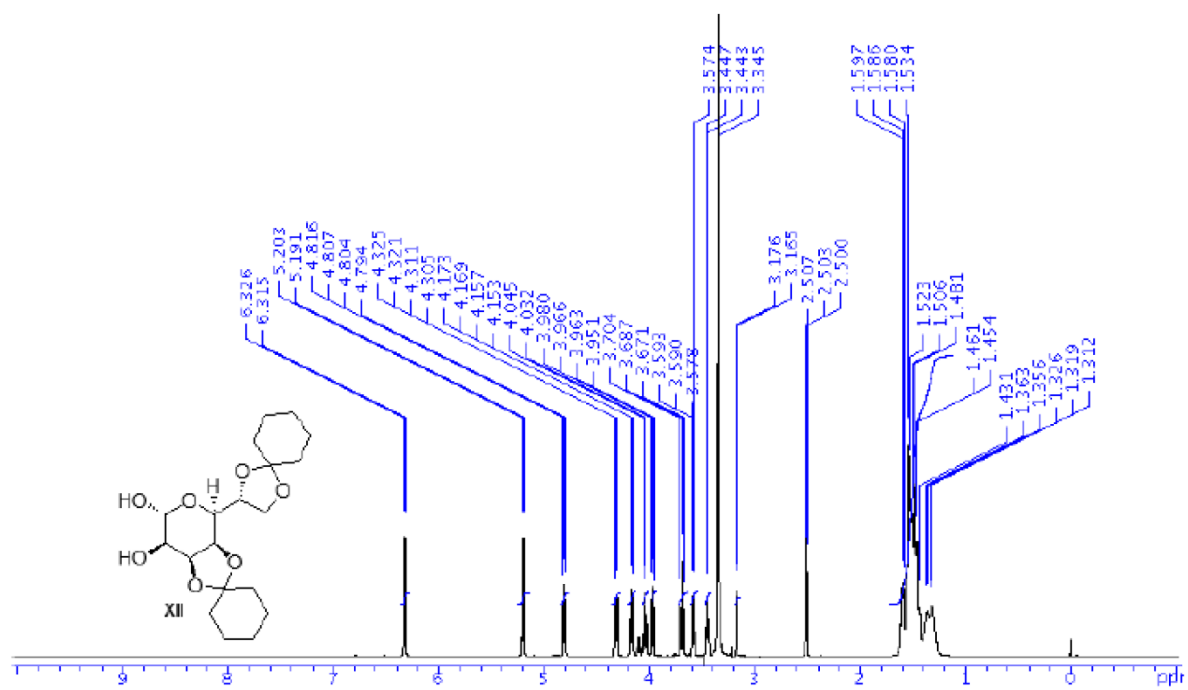
Figure S1 ^1\text{H} NMR of Compound XII
