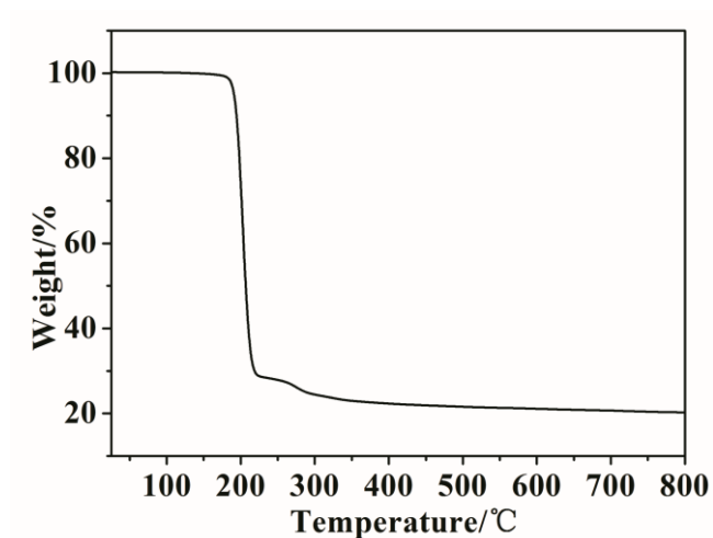
Figure S1. TGA curve of (I).
