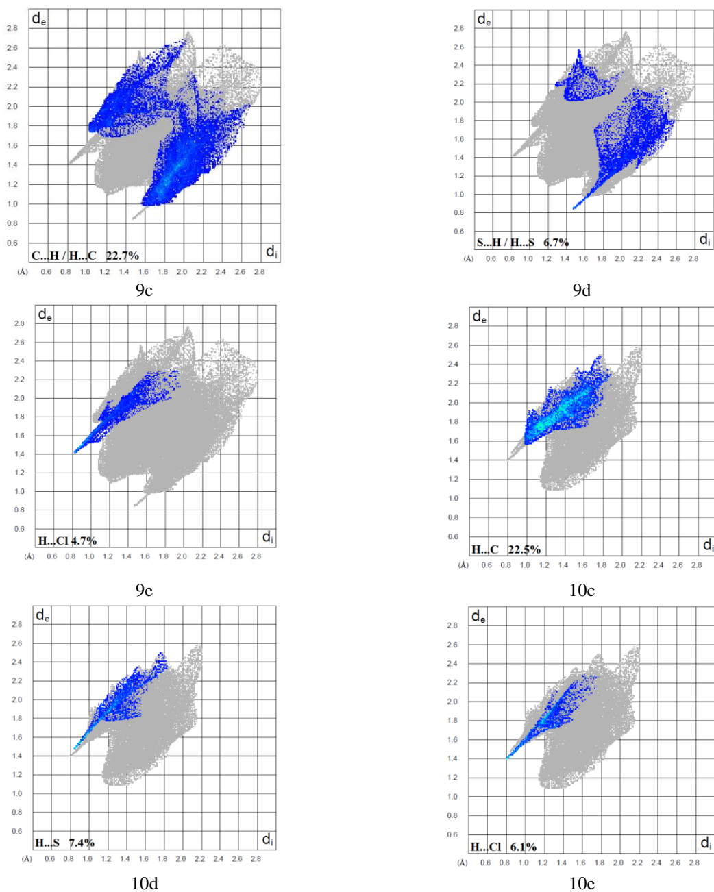
Fig. S1. Divided fingerprint plots, including C...H / H...C (7c), S...H / H...S (7d), N...H / H...N (7e) [for IA], C...H / H...C (8c), S...H / H...S (8d), N...H / H...N (8e) [for IB], C...H / H...C (9c), S...H / H...S (9d), H...Cl (9e) [phosphorothioic triamide molecule of (II)], H...C (10c), H...S (10d) and H...Cl (10e) [for cation of (II)].
