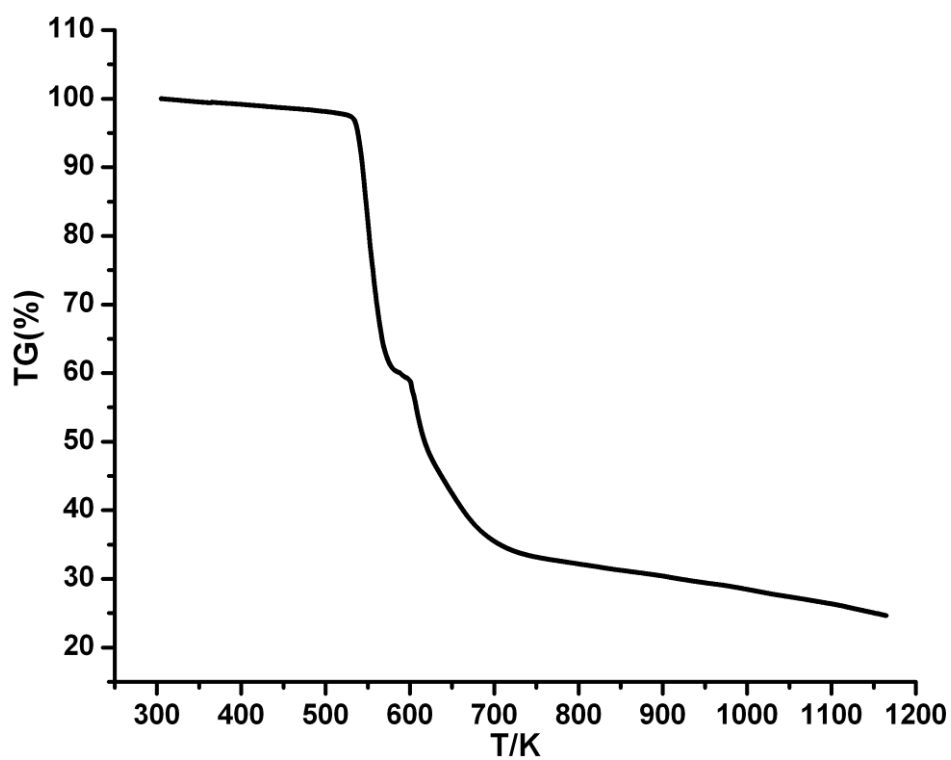
Figure S1 The TG curve of complex I.
