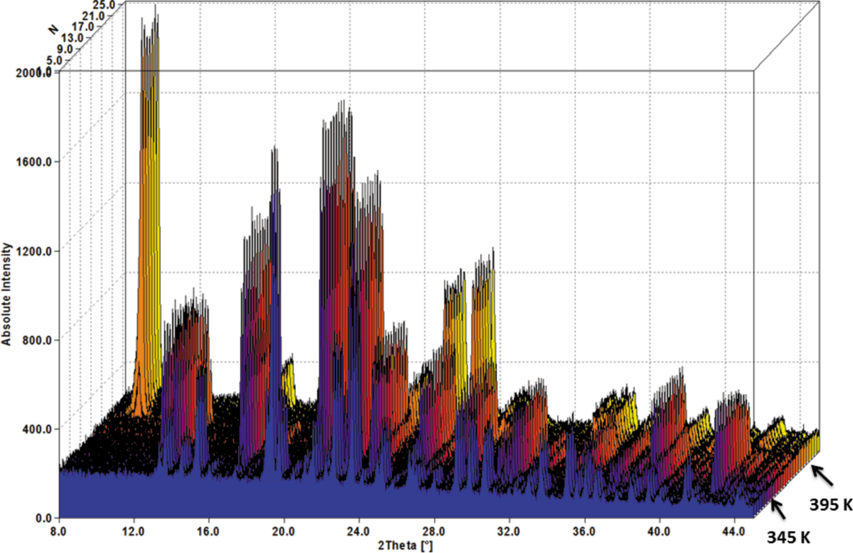
Fig. S2. Variable-temperature powder X-ray diffractograms for the transformation of the zinc glycine ionic complex tetraaquabis(glycine- O )zinc(II) hexaaquazinc(II) bis(sulfate) to the zinc form of complex (I) at ca 343 K, followed by the transformation to the zinc form of complex (II) at ca 393 K.
