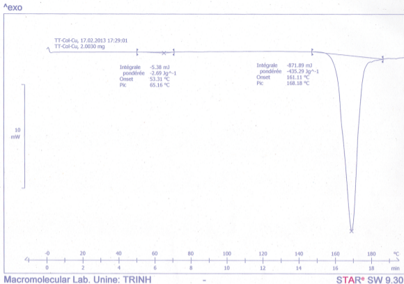
Fig. S1. DSC scan for compound (I); only one transformation is observed.
