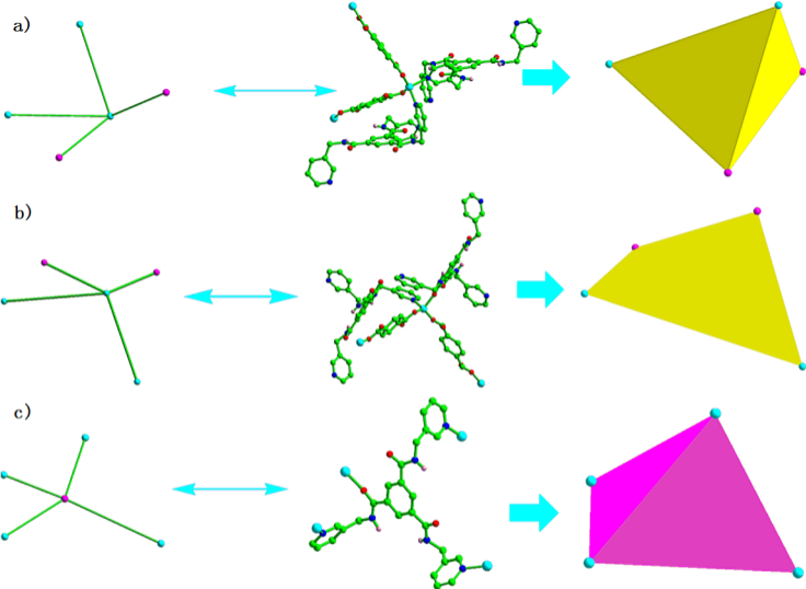
Fig. S1. (a) Schematic description of tetrahedral Zn1 nodes with topological symbol (4.6^2.7^3) , (b) tetrahedral Zn2 nodes with topological symbol (4.6^2.7^2.8) and (c) the 4-connected ligand nodes with topological symbol (4^2.6^2.7^2) .
