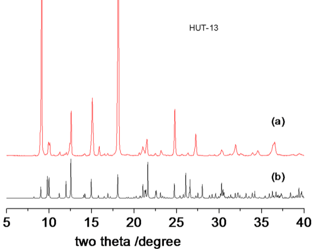
Fig. S3. (a) Measured and (b) simulated powder XRD patterns for HUT-13.
