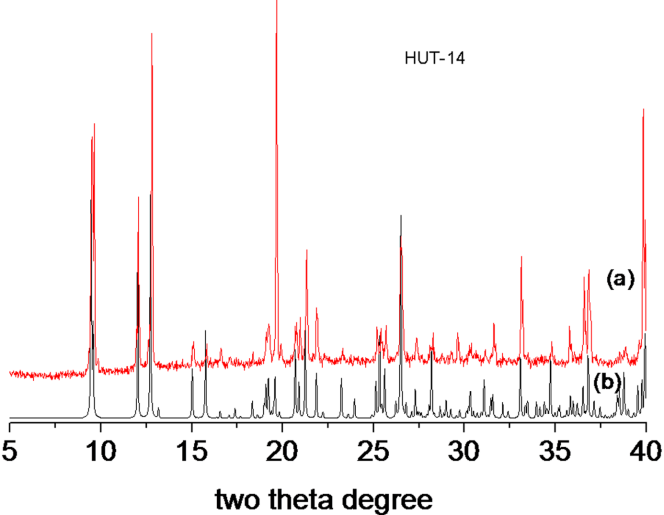
Fig. S4. (a) Measured and (b) simulated powder XRD patterns for HUT-14.
