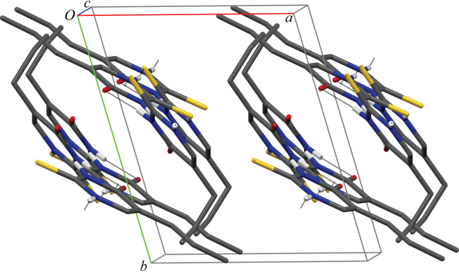
Supplementary figure. A packing diagram for (I), showing the tubular arrangement of the chains. Hydrogen bonds are shown as dashed lines.
