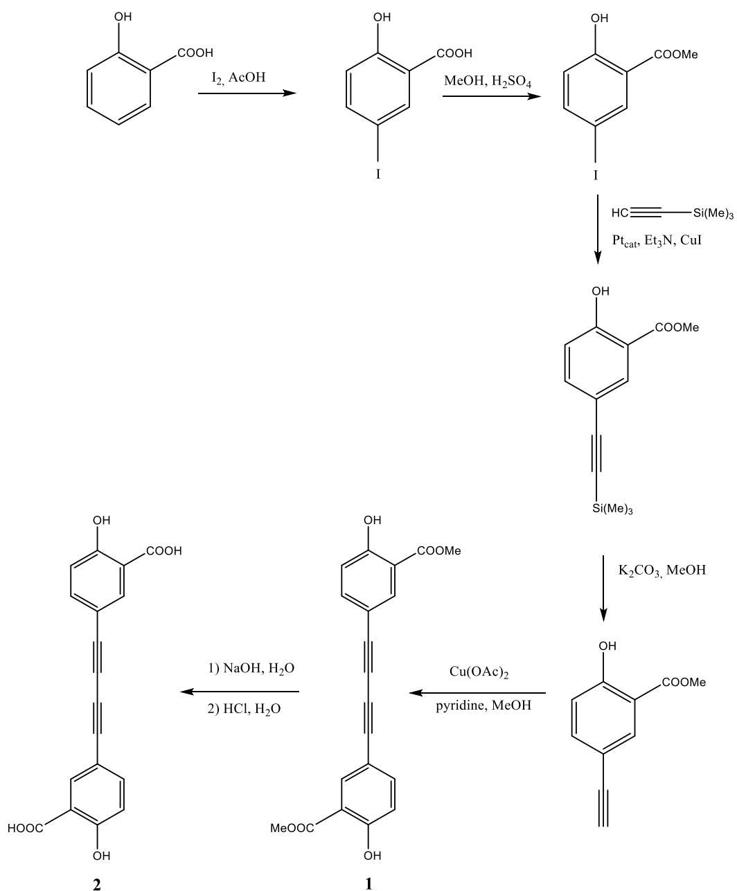
Figure S2 – Scheme for the synthesis of 5,5'-(1,3-butadiene-1,4-diyl)bis(2-hydroxybenzoic acid)
