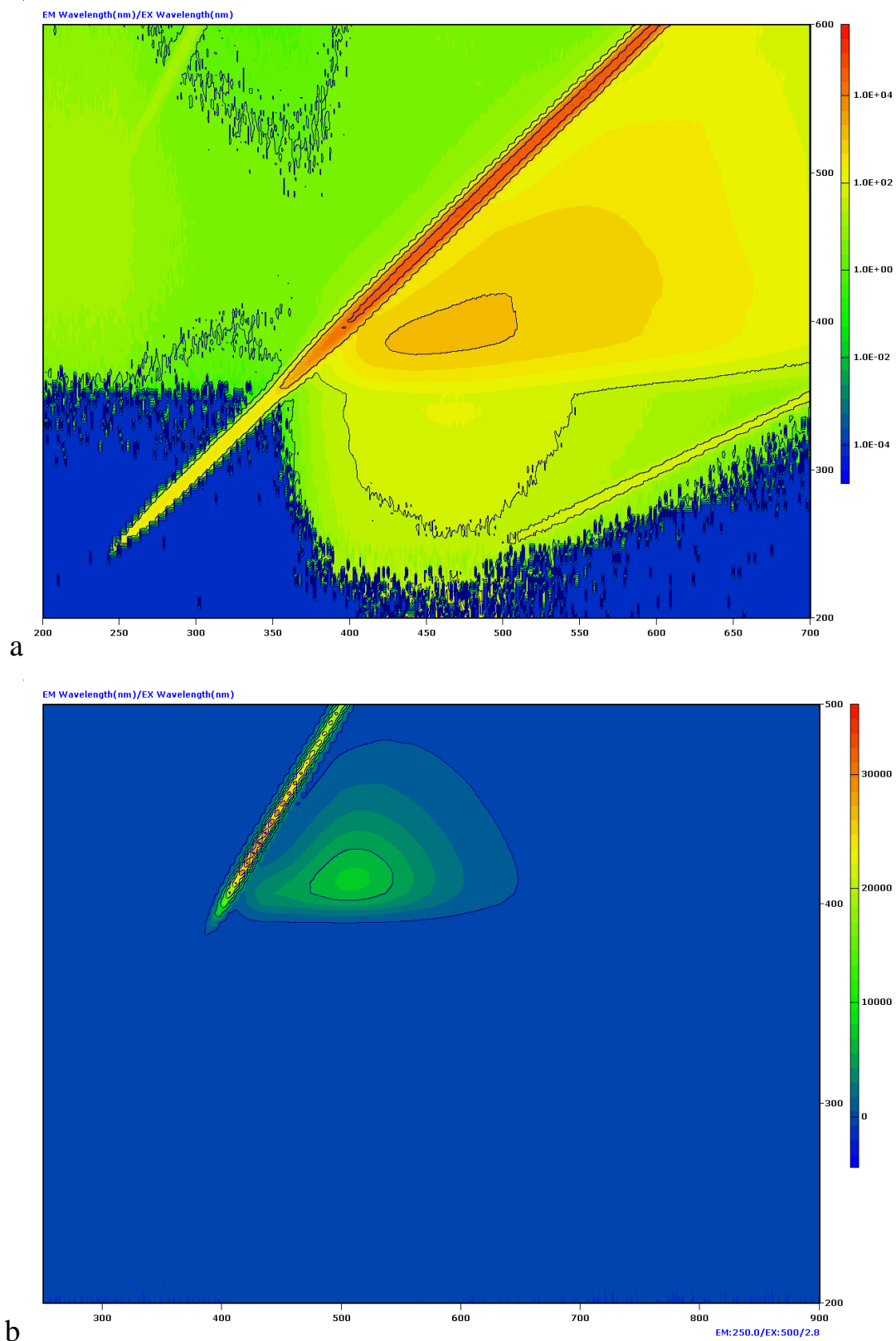
Figure S3 – Intensity distribution diagram of compounds 1 (a) and 2 (b) in DMSO solution
