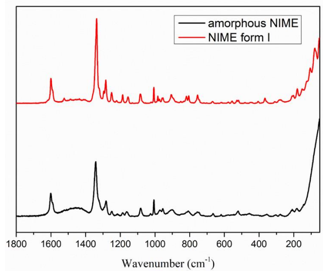
Figure S1. Raman spectra of amorphous and form I of nimesulide.
