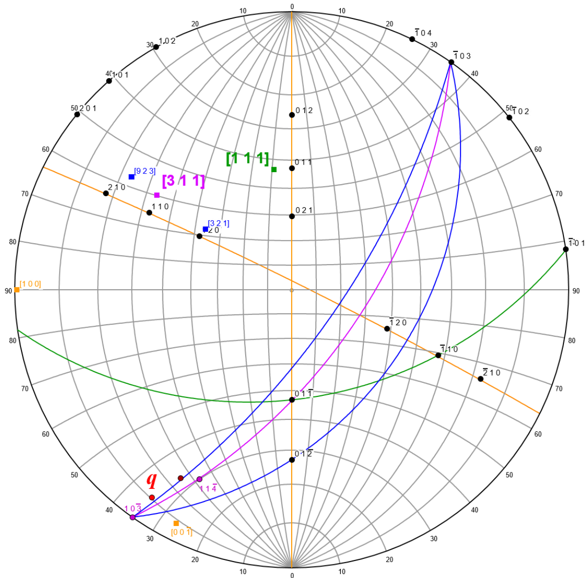
Figure S1 Stereographic net showing the q -vector of the andesine (labelled with q ), some directions, and some (hkl) planes and their poles.
