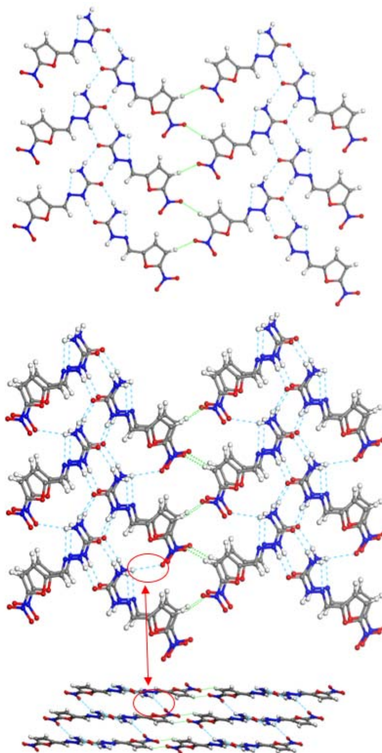
Figure S2 Single crystal structure of 5-nitrofurazone form \beta (CCDC references: 1444950).
