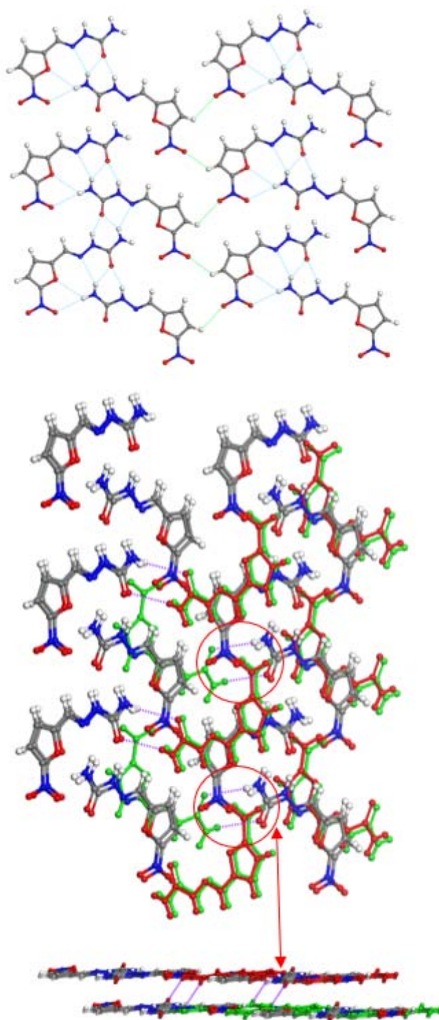
Figure S1 Single crystal structure of 5-nitrofurazone form \alpha (CCDC references: 1292340).
