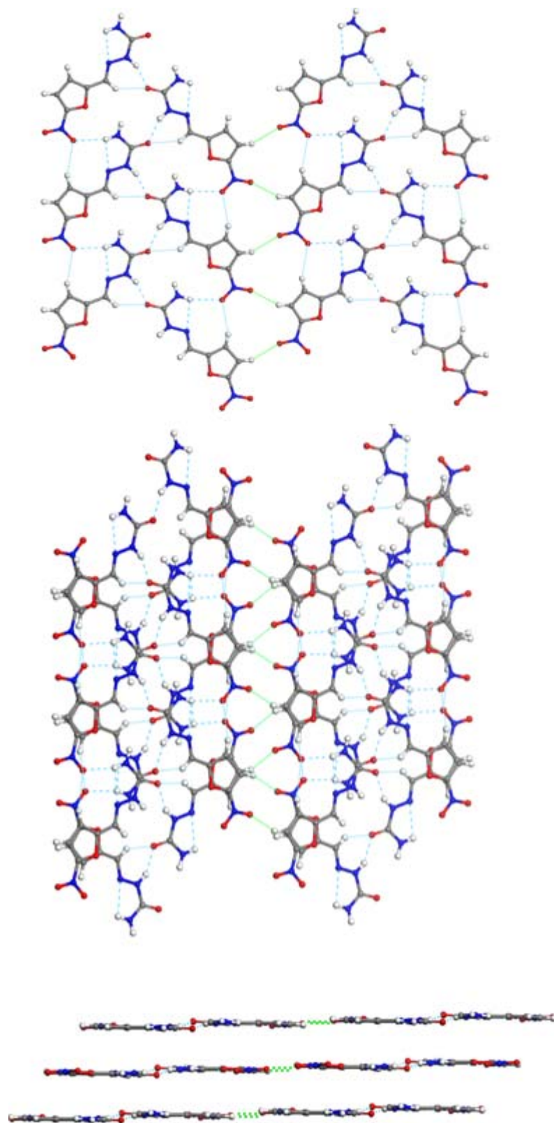
Figure S3 Single crystal structure of 5-nitrofurazone form \gamma (CCDC references: 1444951).
