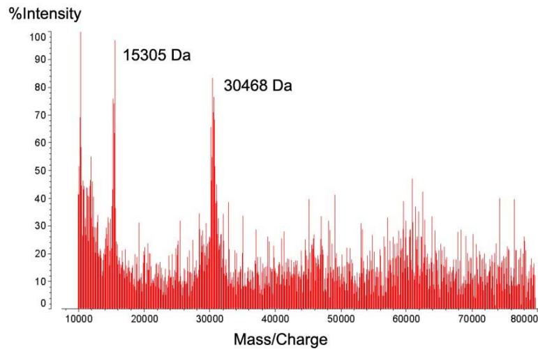
Fig S2. The result of mass spectrum. The mass of one human Calbindin-D28k molecule with one and two charges were labeled as 30468 Da and 15305 Da respectively, which indicated that the actual molecular weight of Calbindin-D28k should be 30.5 kDa.
