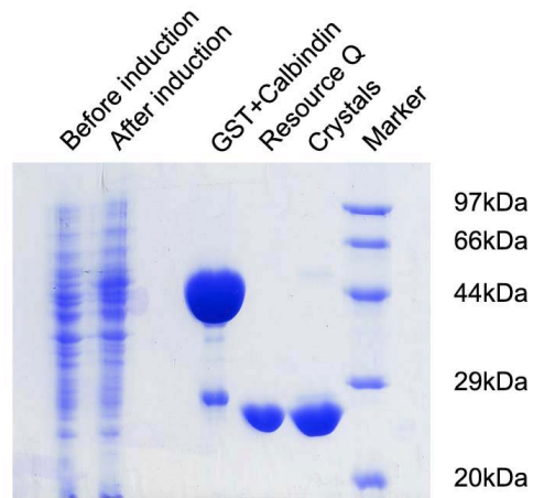
Fig S1. The result of electrophoresis. The lanes and molecular weight of protein markers were labeled respectively.
