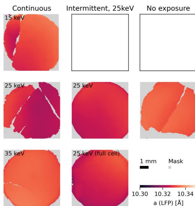
Figure S7 Lattice parameter a (LFP) obtained from Rietveld refinements of PXR mapping of LFP electrode pellets.
