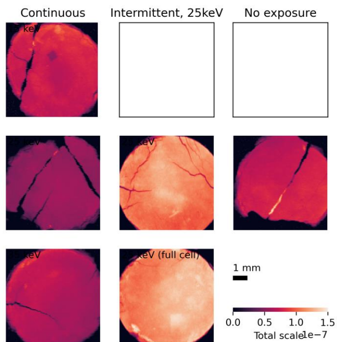
Figure S6 Total scale factors obtained from Rietveld refinements of PXR mapping of LFP electrode pellets.
