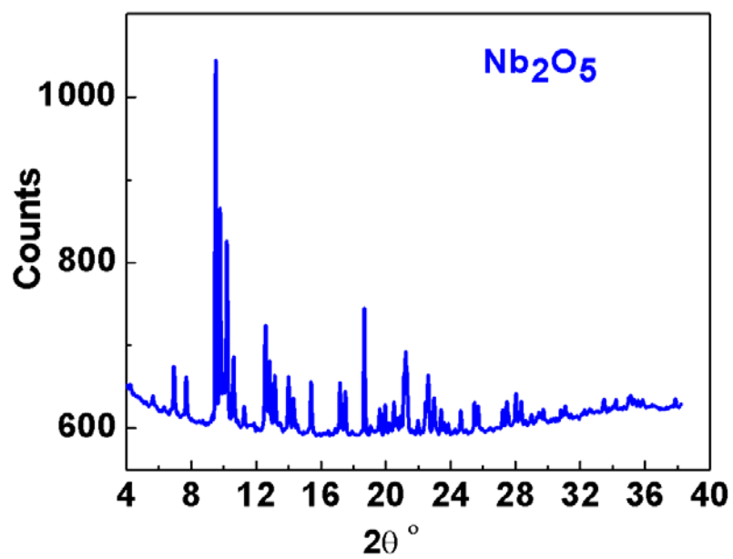
Figure S1 XRD spectrum for Nb 2 O 5 , measured at Indus-2
