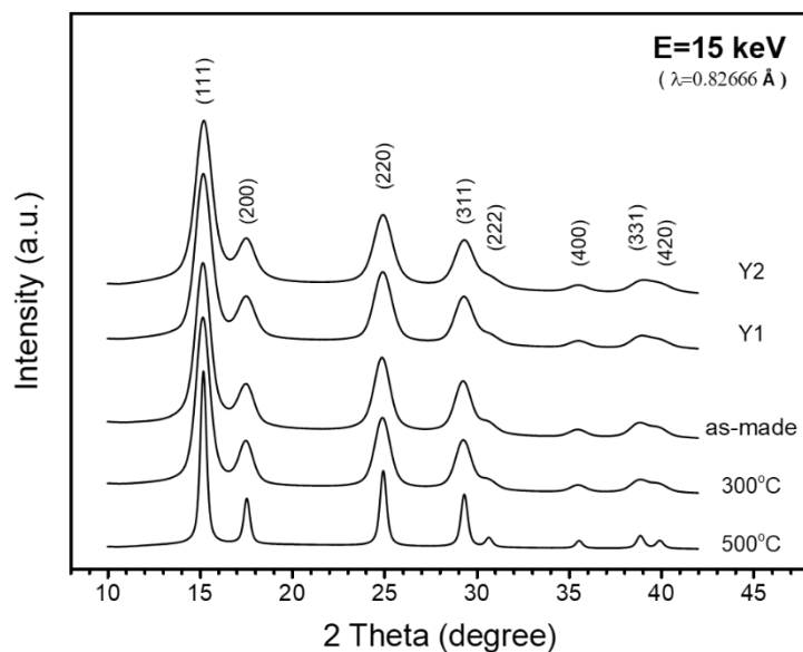
Figure S1 XRD patterns of CeO 2 samples annealed at different temperatures and Y-doped CeO 2 sample Y1 and Y2. Curves have been shifted vertically for the sake of clarity.
