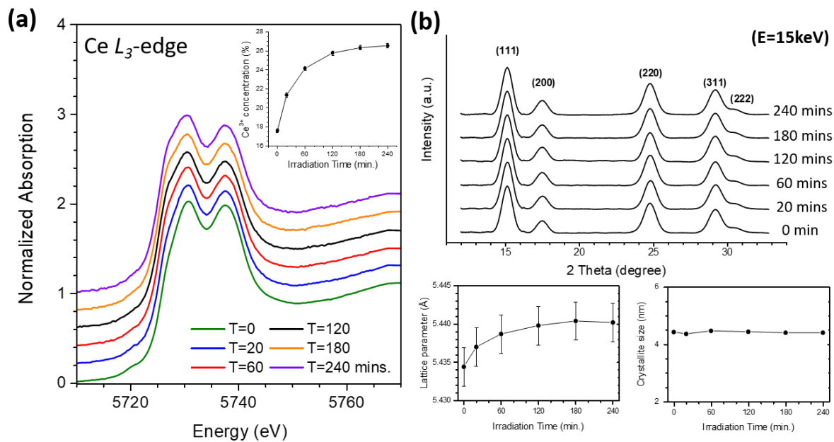
Figure S2 (a) Ce L 3 -edge XANES and (b) XRD patterns of CeO 2 samples with different x-ray irradiation times.
