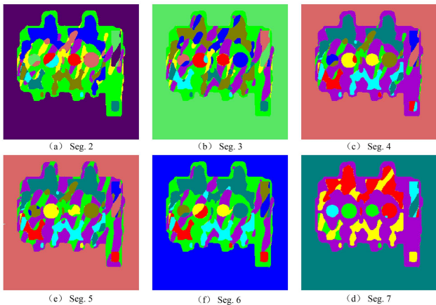
Figure S1 Segment results of the SART-TV reconstruction of the Phantom 3 with an angular range of \alpha = 130^\circ (supplemental information to Fig. 10).
