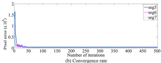
Figure S2 Convergence rate of the different segment results as an initial input of the MDART (supplemental information to Fig. 10).
