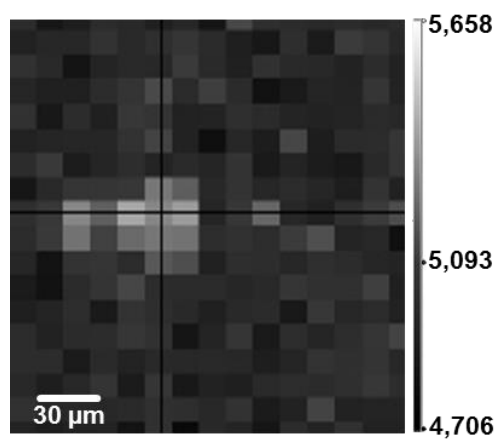
Figure S1 Scan of detector against second zone plate in off-axis CSTXM setup (710 eV). The investigated sample was a magnetite-functionalized PVA-based microballoon. Even with a dwell time of 1 s the fluorescence signal is very low compared with background intensity.
