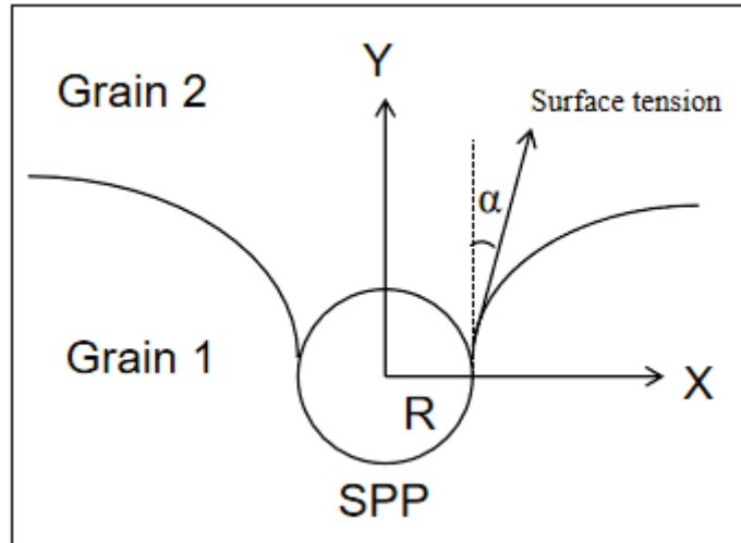
Fig. S1. Interaction between the SPP and a high angle boundary
