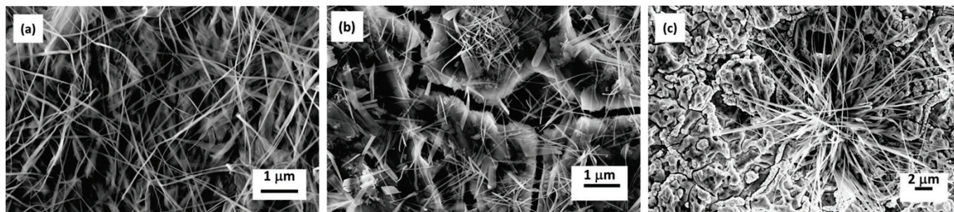
FIGURE SI.2. FESEM top-view images of anodized German silver alloy in 1M NaHCO 3 for 30 minutes at (a) 6 V, (b) 10 V, and (c) 12 V.
