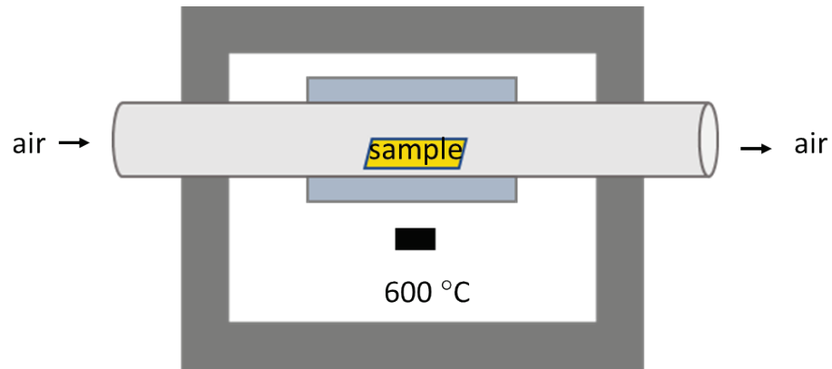
FIGURE SI. 3. Schematic diagram of Thermal treatment of German silver alloy at 600 °C for 1hr in air.
