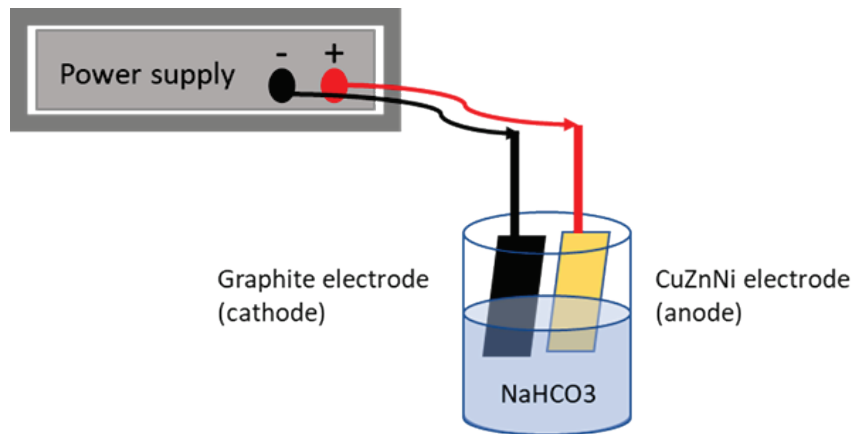
FIGURE SI.1. Schematic diagram of anodization treatment of nickel silver alloy as the anode in 1M NaHCO 3 solution at room temperature.
