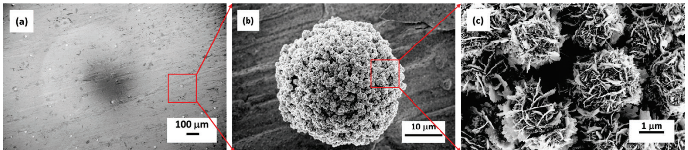
FIGURE SI.4. FESEM top-view images of thermally treated German silver alloy at 600°C for 1hr in air.
