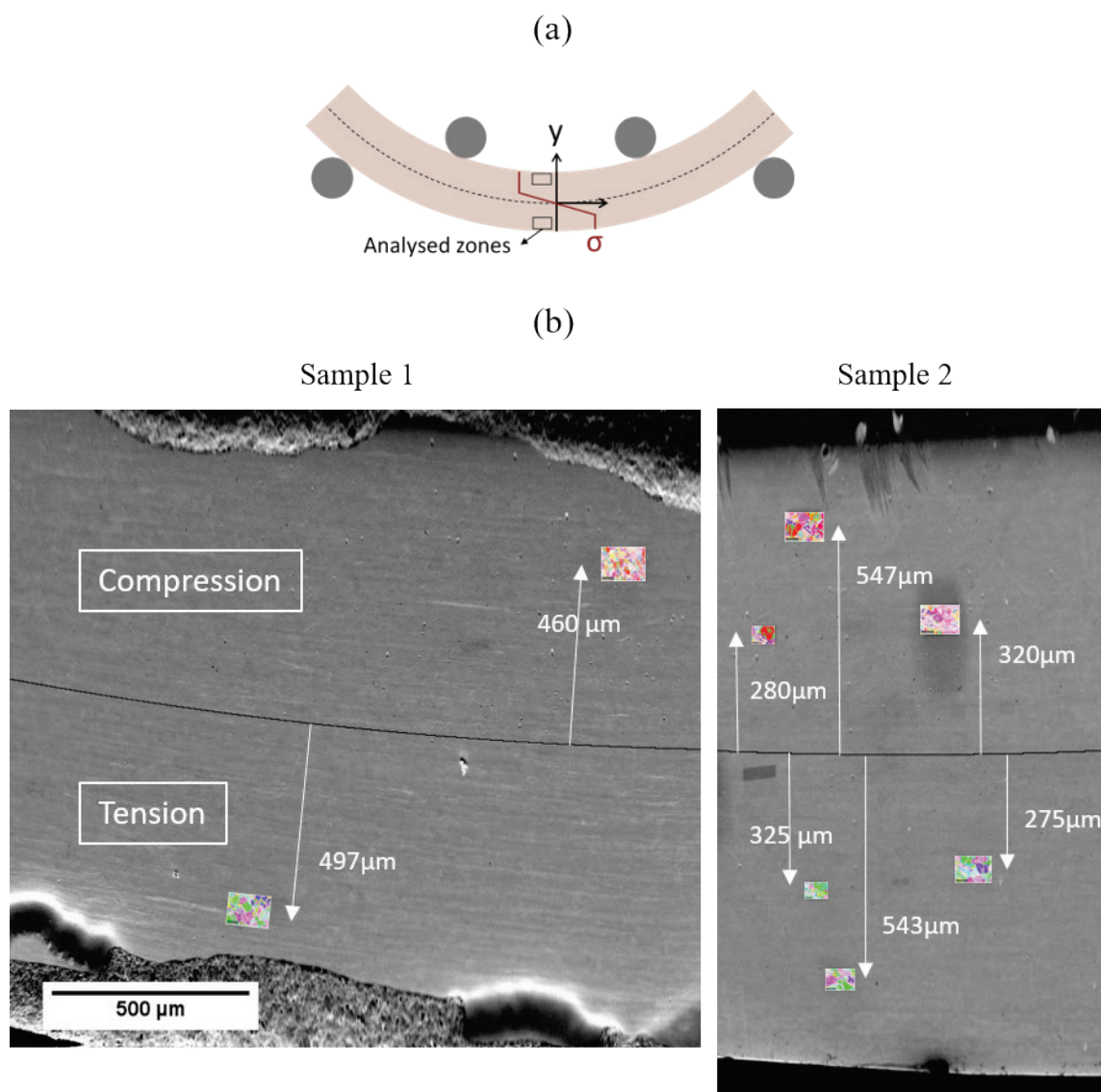
Figure S2 Analysed zones (a) schematic of the beam (b) corresponding SE images and superimposed EBSD maps, with their distance from the neutral line.
