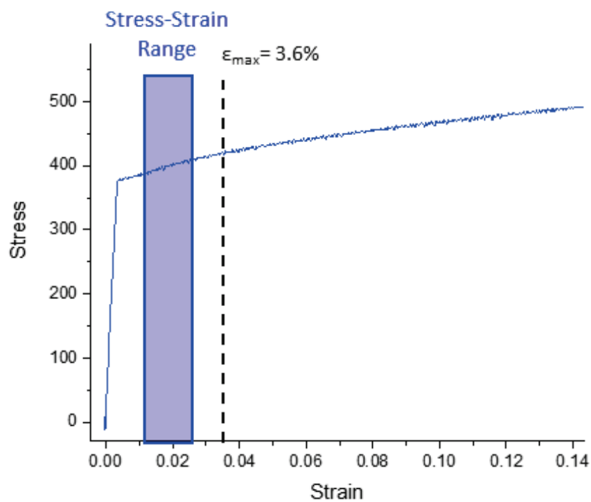
Figure S1 Tension stress-strain curve of the studied alloy in the fcc phase at room temperature, the shaded area corresponding to the stress and strain range of the analysed zones in tension and symmetrically in compression.
