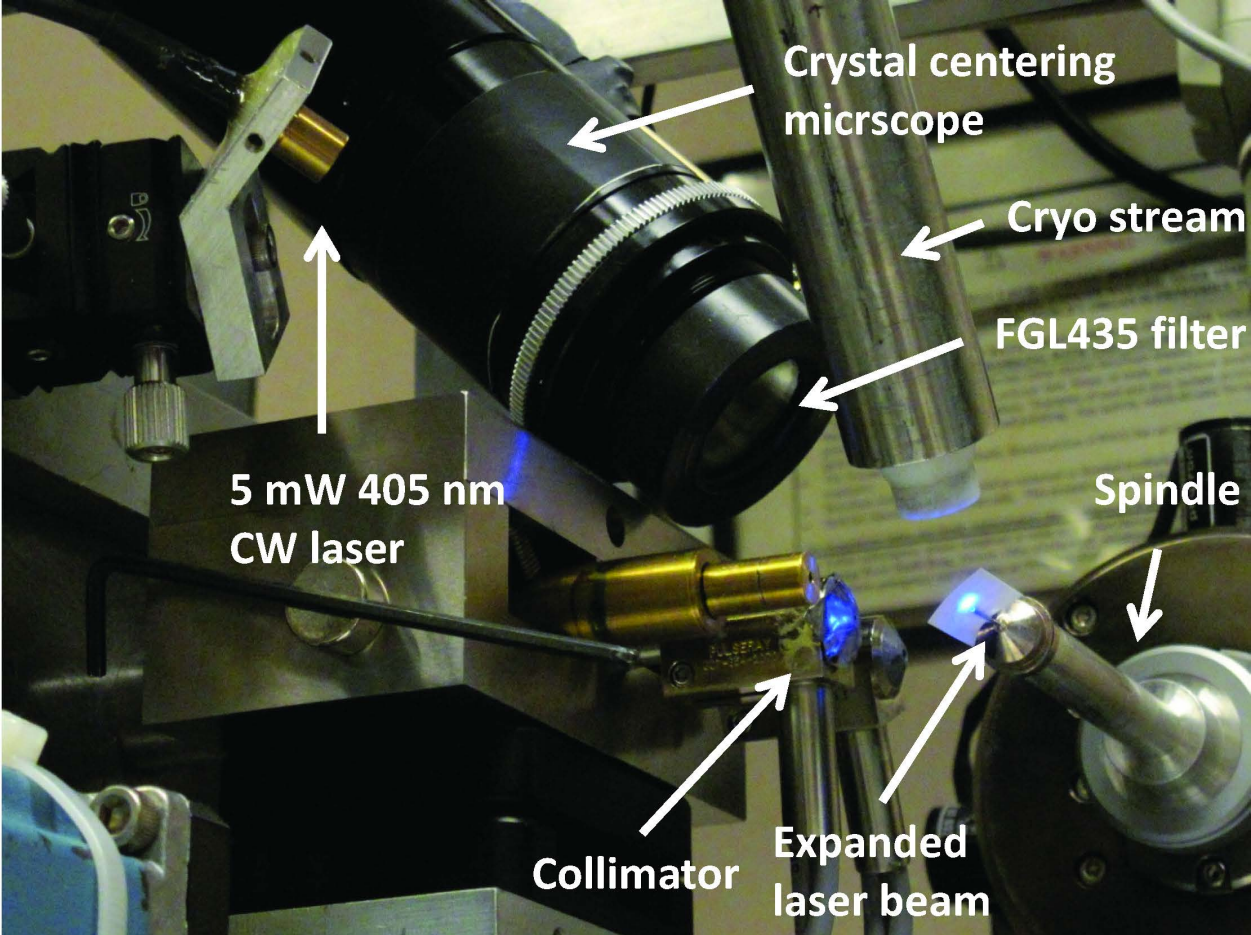
Figure S4 Fluorescence microscopy set-up in the A1 station at CHESS utilizing a 5 mW 405 nm CW laser and an FGL435 Schott glass filter. The laser beam is aligned to the center of rotation of the spindle via a piece of paper mounted onto an ALS type base.
