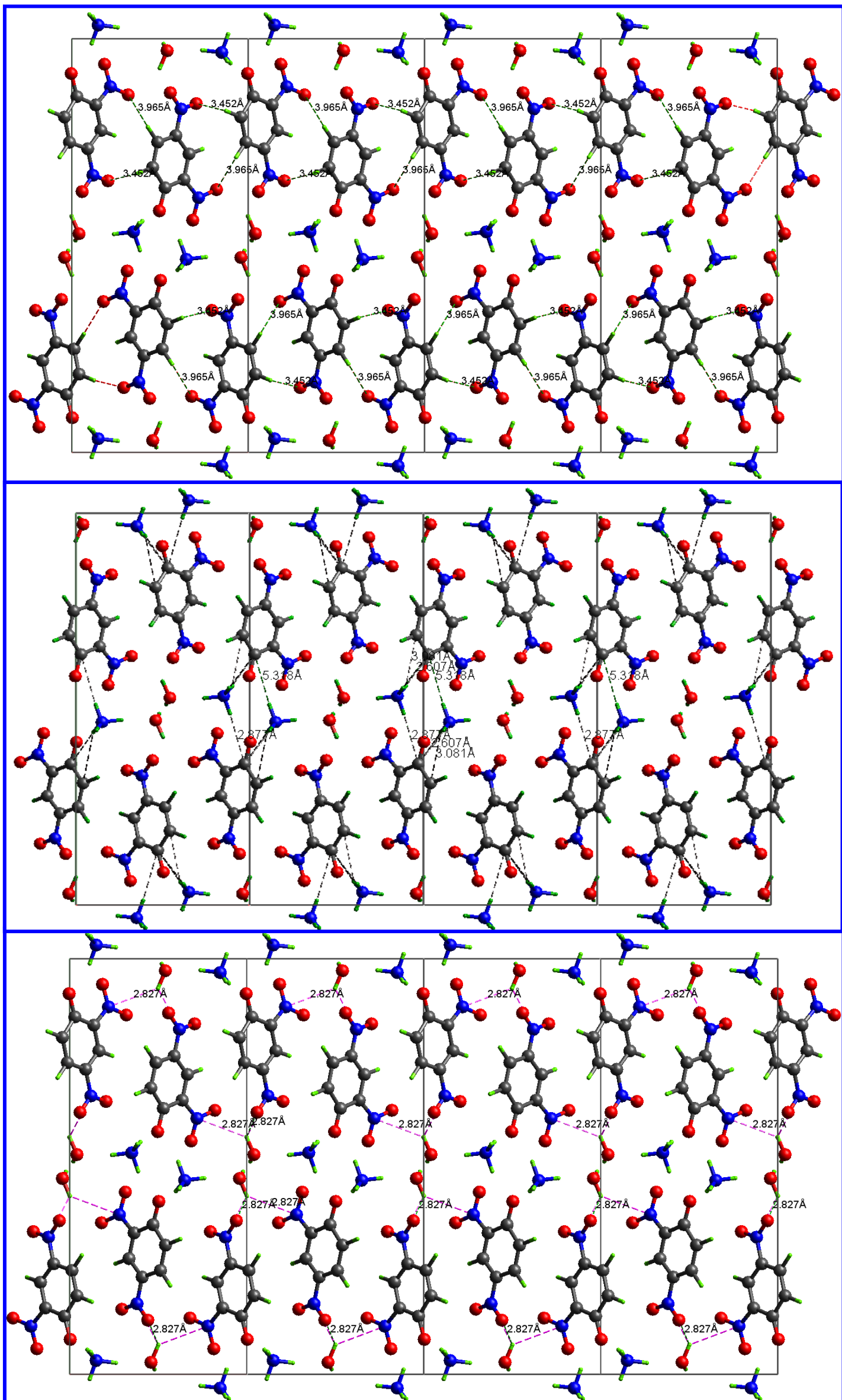
Fig. S1. C-H...O, N-H... \pi and O-H...N interactions
