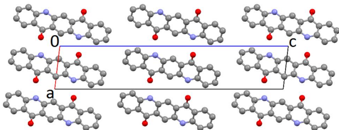
Fig. S2. Crystal structure of quinacridone
