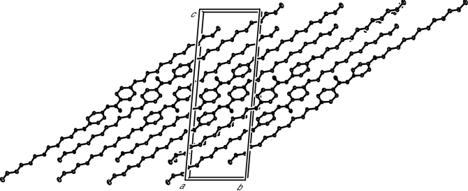
Packing diagram for (I), viewed down the a axis.
