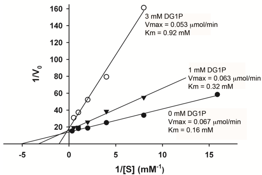
Figure S1 Lineweaver-Burk plot of L-Galactitol-1-P oxidation in the presence of 0, 1 and 3 mM D-Galactitol-1-P (DG1P).
