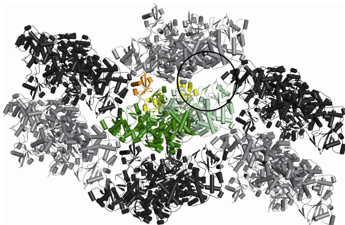
Figure S1 Crystal packing. Crystal packing analysis illustrates that the Ub(t) (orange) contacts two Uba1 symmetry mates (grey and black), thus stabilizing it and presumably leading to its visibility. At the equivalent position in the second Uba1 complex the presence of Ub(t) is prevented (circle).
