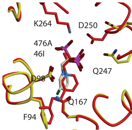
Supplementary Figure S2. Structural overlap of LmFPPS in the complexes with 476A (red) and with 46I (yellow). Residues of the allylic site that have different conformations are shown. The inhibitor bound in each complex is shown. Metals are not shown for clarity.
