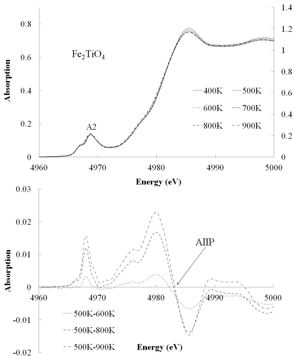
Figure S5 Ti K-edge XANES spectra of \text{Fe}_2\text{TiO}_4 at each temperature.
