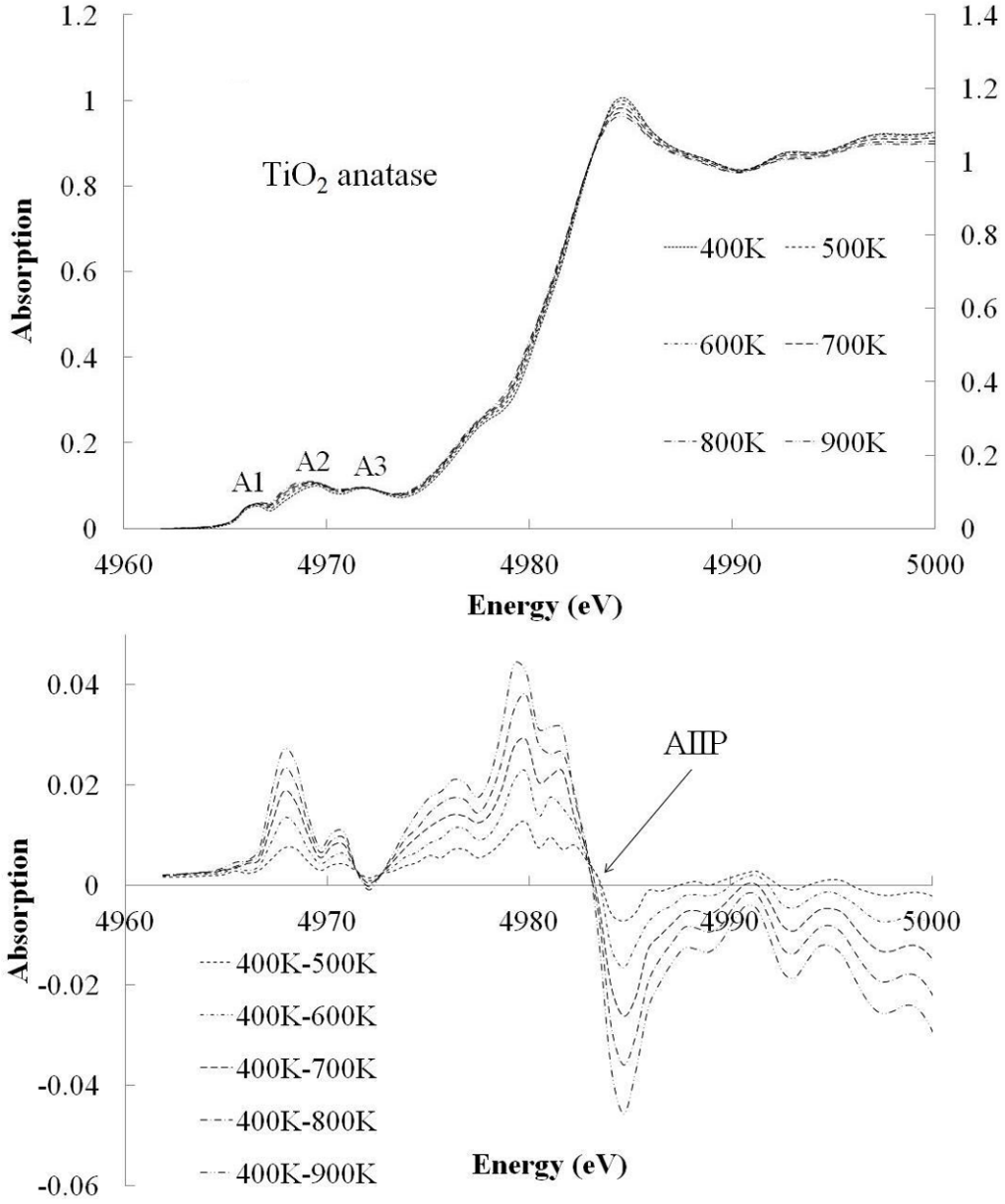
Figure S3 Ti K-edge XANES spectra of TiO 2 anatase at each temperature.
