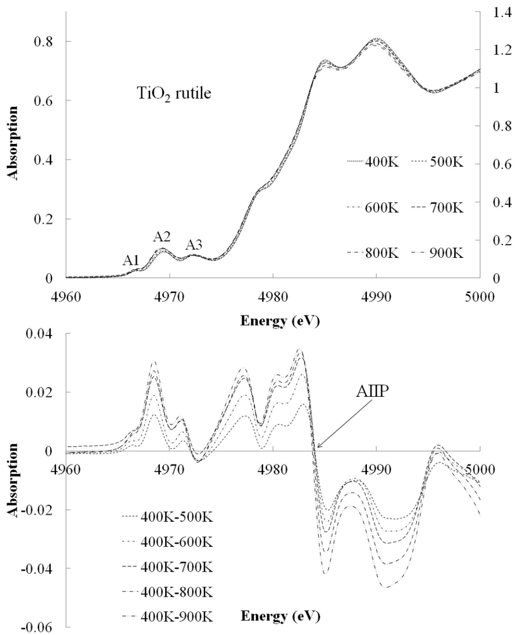
Figure S2 Ti K-edge XANES spectra of TiO 2 rutile at each temperature.
