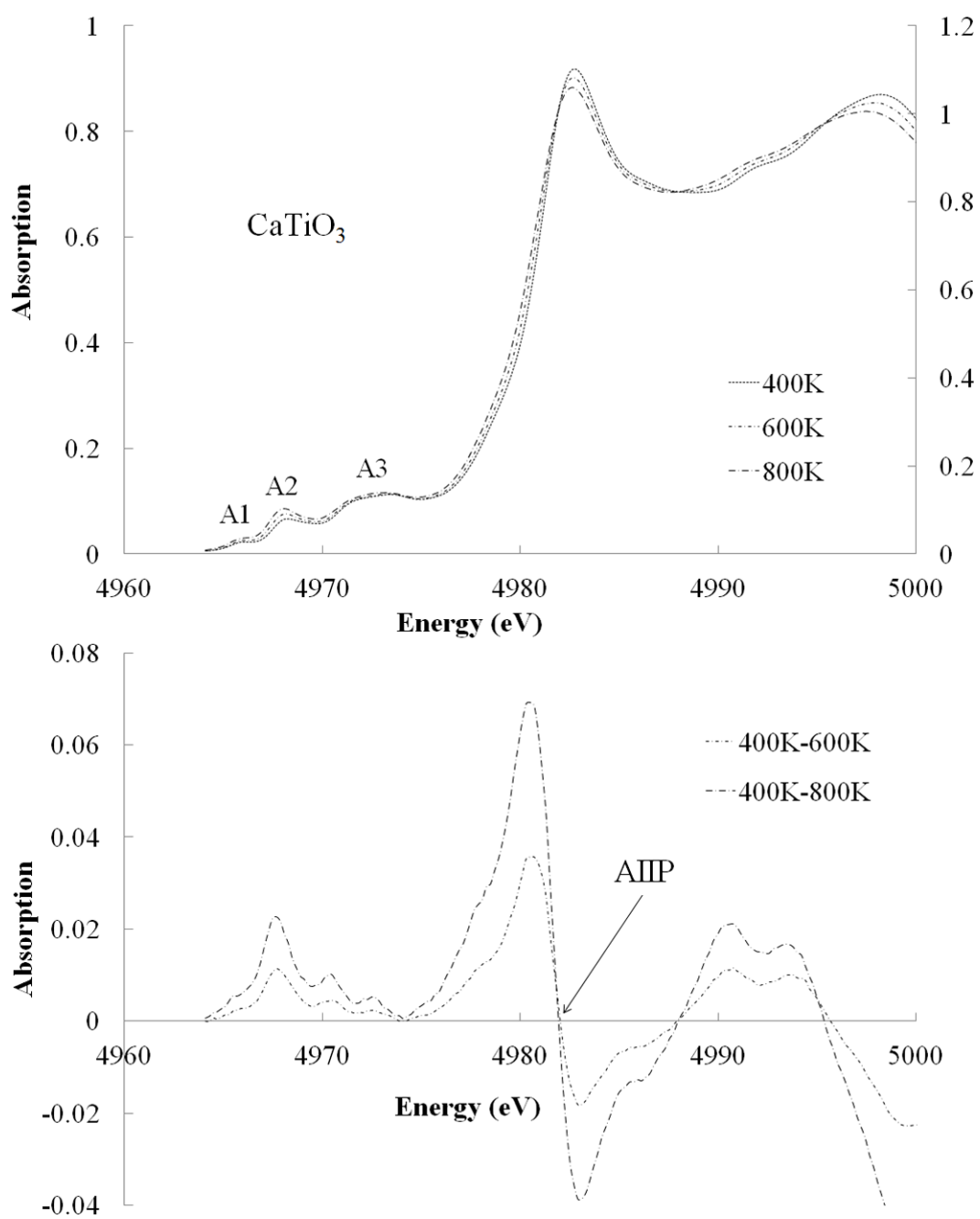
Figure S1 Ti K-edge XANES spectra of \text{CaTiO}_3 at each temperature.
