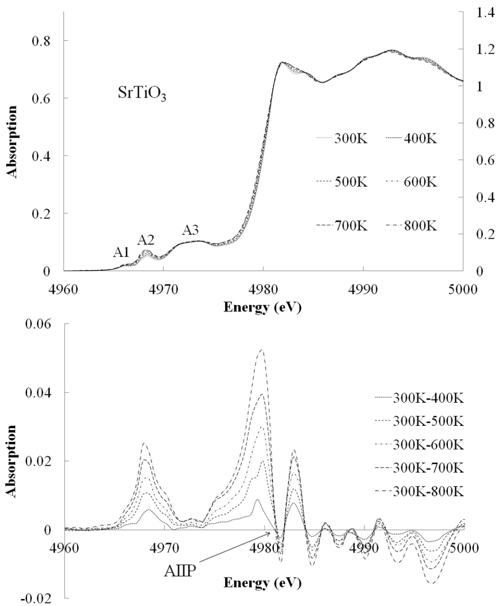
Figure S4 Ti K-edge XANES spectra of SrTiO 3 at each temperature.
