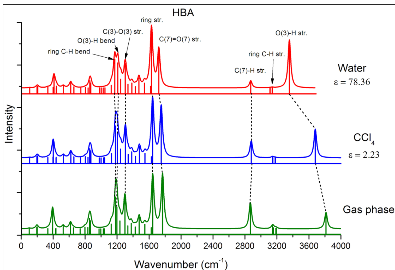
Figure 2S. Solvent effect of HBA.
