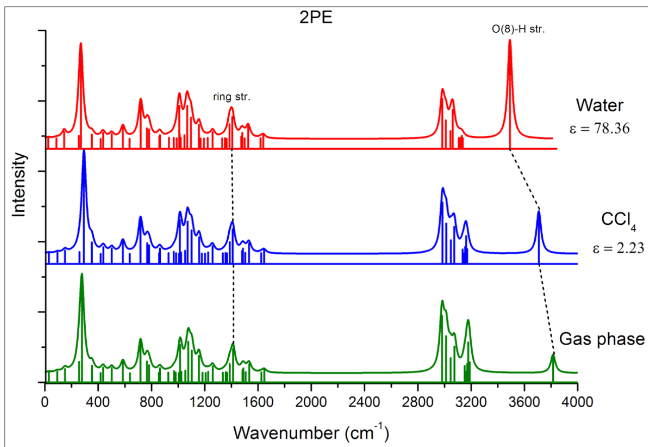
Figure 1S. Solvent effect of 2PE.
