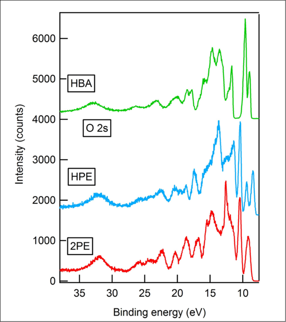
Figure 3S. Complete experimental valence vertical ionization spectra.
