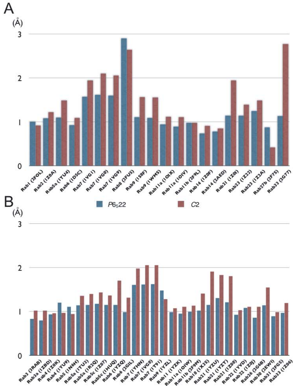
Supplementary Figure 2. Structural comparison with Rabs. R.m.s.d. values for the superimposition of Rab GDP-form ( a ) and Rab GTP-form ( b ) structures. The values were calculated for the core domain excluding the switch I, switch II and interswitch elements, in Å, for both P6_522 and C2 space groups. The values for the comparison with the P2_12_12_1 structures are highly identical to those for the C2 structure. The PDB accession numbers used for the alignment are indicated.
