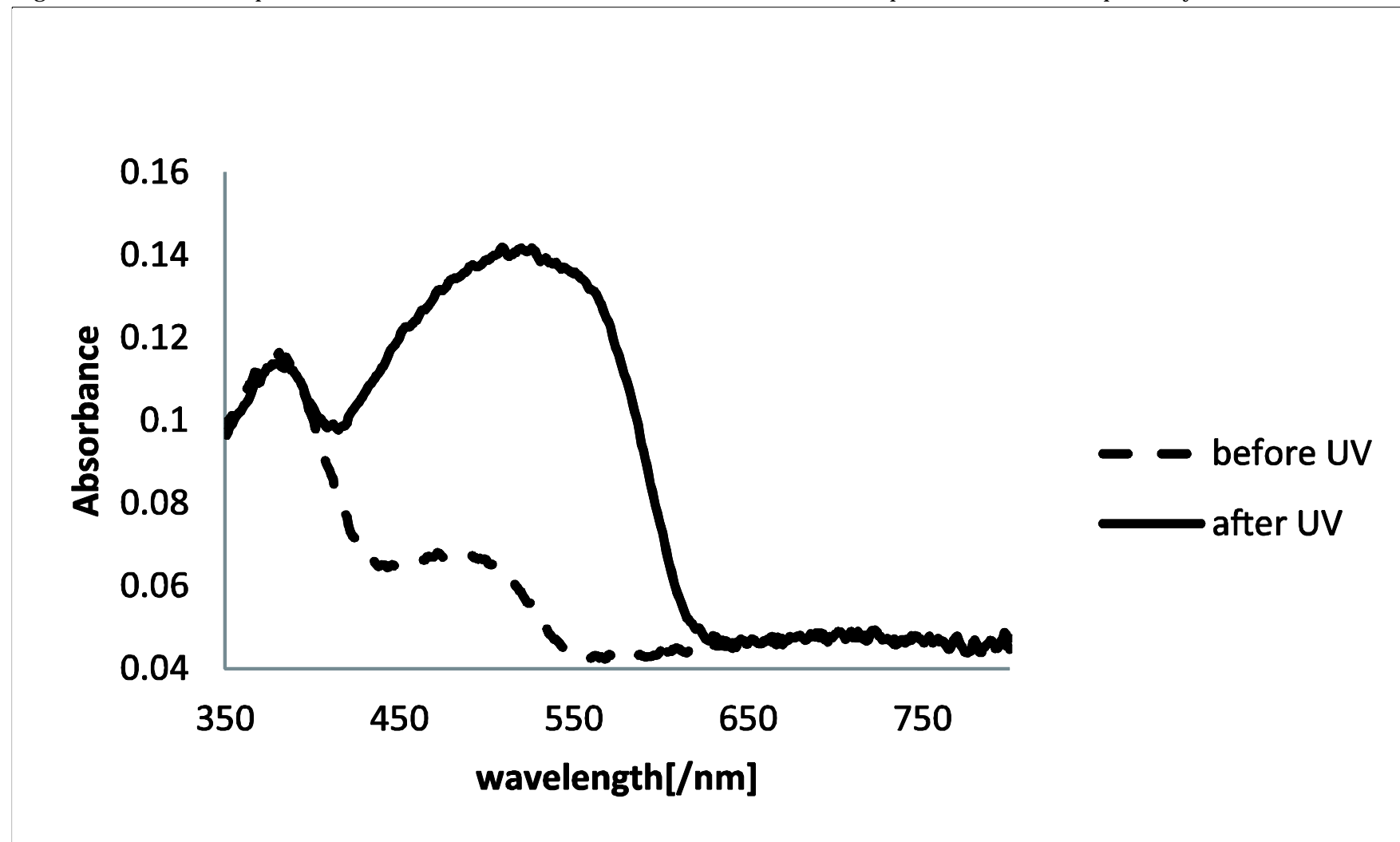
Figure S4 Reflectance spectra for 5. Dashed and full curves indicate before and after photoirradiation, respectively.
