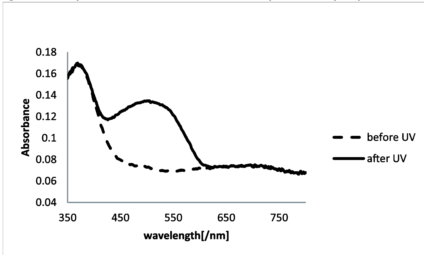
Figure S2 Reflectance spectra for 3 . Dashed and full curves indicate before and after photoirradiation, respectively.
