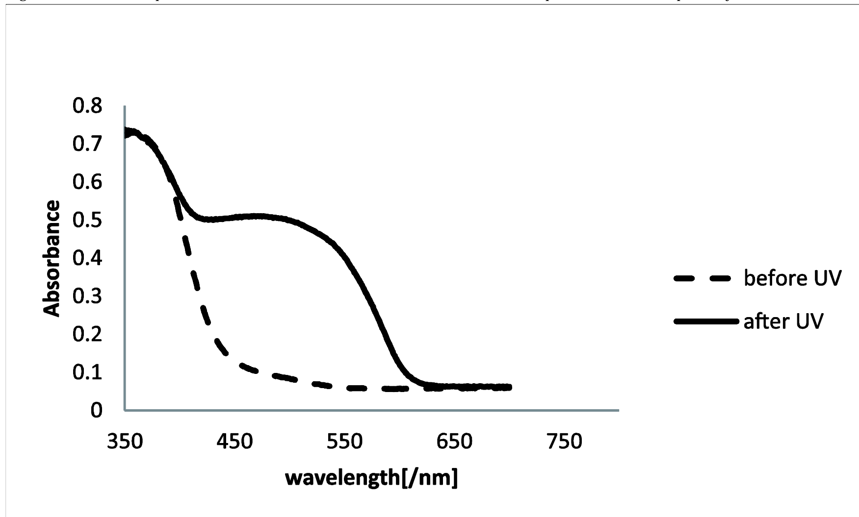
Figure S1 Reflectance spectra for 2 . Dashed and full curves indicate before and after photoirradiation, respectively.
