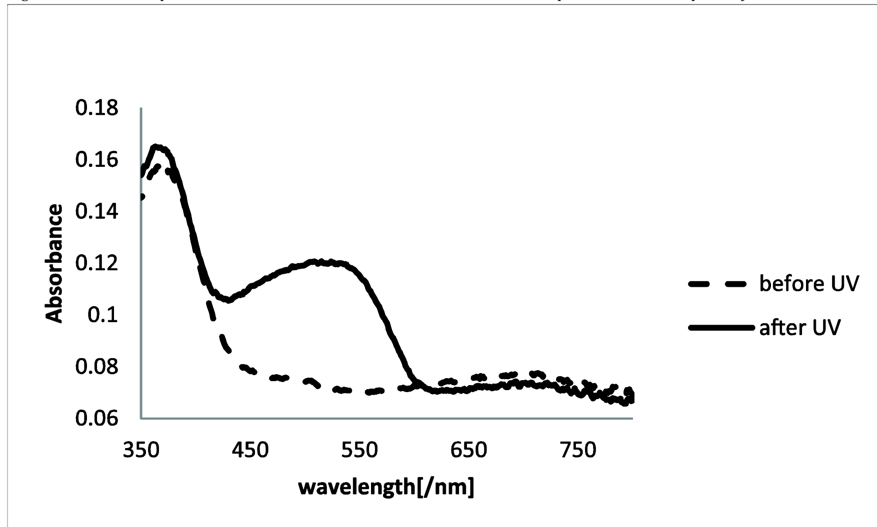
Figure S3 Reflectance spectra for 4 . Dashed and full curves indicate before and after photoirradiation, respectively.
