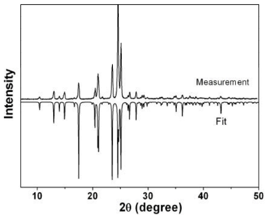
Figure 2S. The powder XRD (PXRD) pattern of I at room temperature. The lower pattern is simulated from the single crystal structure.
