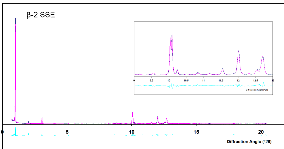
Figure 5 Rietveld refinement of \beta -2 SSE with difference trace of the measured and calculated patterns
