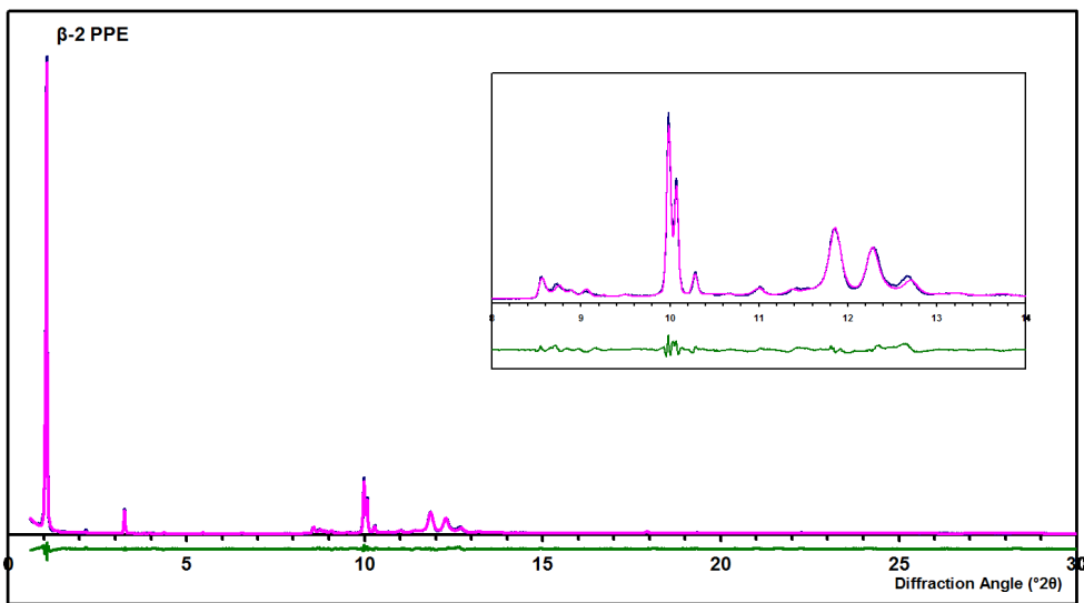
Figure 4 Rietveld refinement of \beta -2 PPE with difference trace of the measured and calculated patterns
