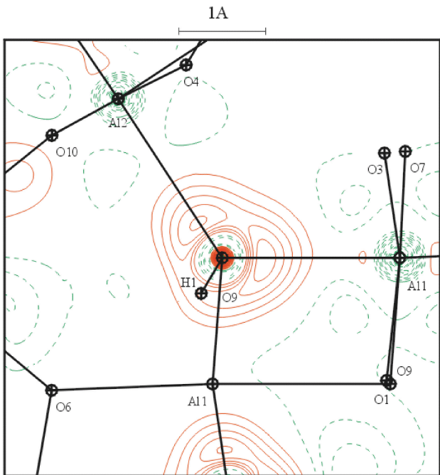
Static deformation map in the plane A12-O9-A11. Contours as in Fig. S3.
