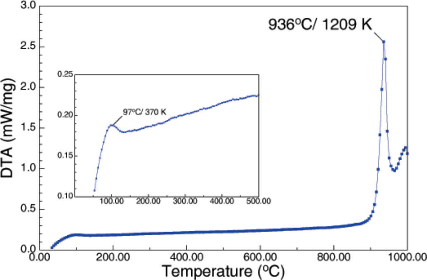
Differential thermal analysis of \text{Li}_2\text{Ge}_4\text{O}_9 ; the inset shows the low-temperature region on an extended scale
