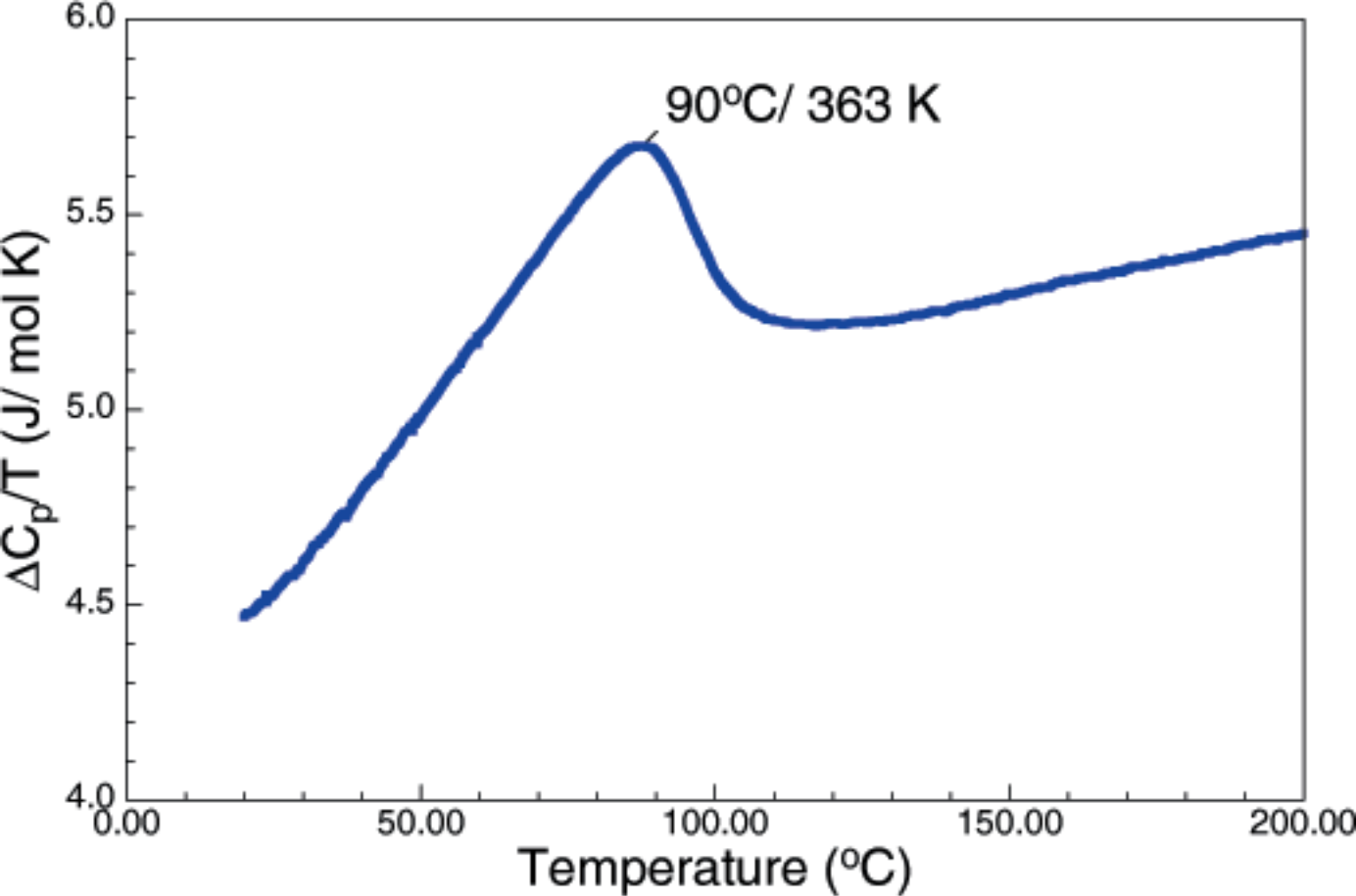
Specific heat measurement of \text{Li}_2\text{Ge}_4\text{O}_9 .
