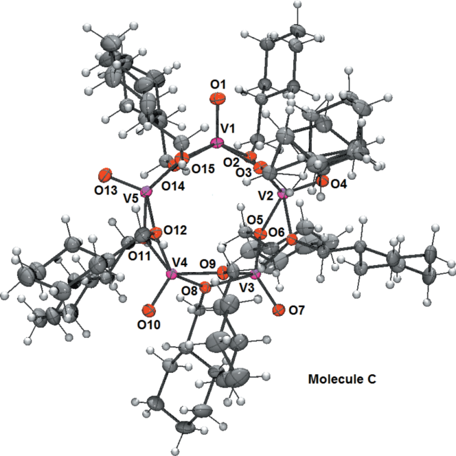
Fig. 2S. The molecular structure of molecule C of (I), with displacement ellipsoids drawn at the 30% probability level.
