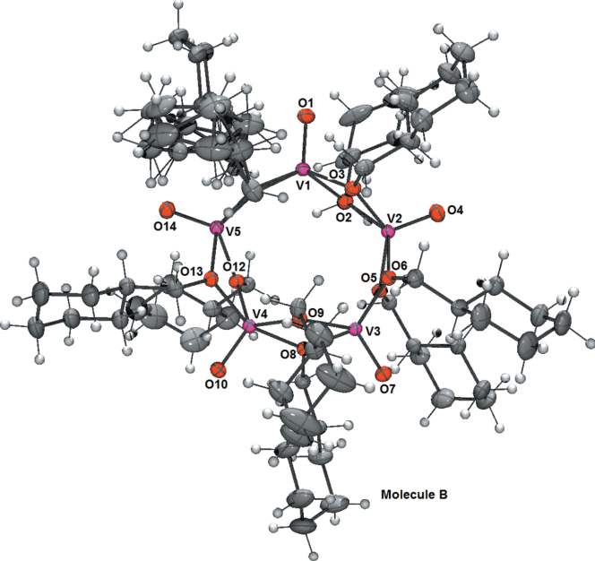
Fig. 1S. The molecular structure of molecule B of (I), with displacement ellipsoids drawn at the 30% probability level.
