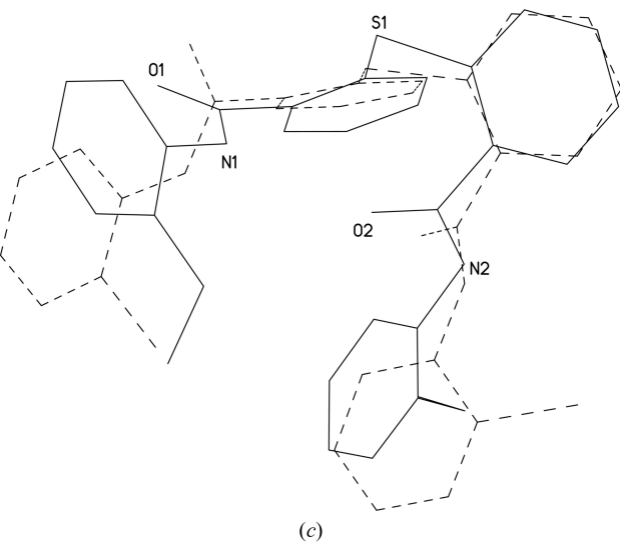
Supplementary Figure 1. Overlays of the molecules in pairs, showing (a) (Ia) (dashed) and (Ib), (b) (Ia) and (Ic) (dashed), and (c) (Ib) and (Ic) (dashed). H atoms have been omitted.
