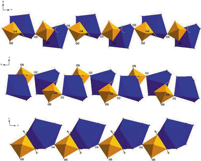
Supplementary Fig. 5. Bipolyhedral chains running in three different directions.
