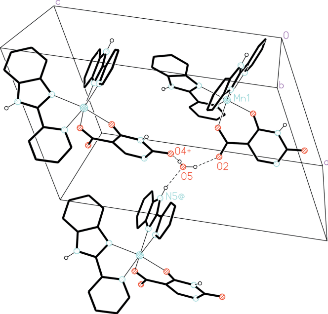
Supplementary Figure S3. A view of the 3[\text{Mn}(\text{Huca})(\text{Hpybim})_2]/\text{H}_2\text{O} aggregate formed through the lattice water molecules of (I). Atoms labelled with a plus sign (+) and an at sign (@) are at the symmetry positions (x, -y+3/2, z+1/2) and (x+1, -y+3/2, z+1/2) , respectively.
