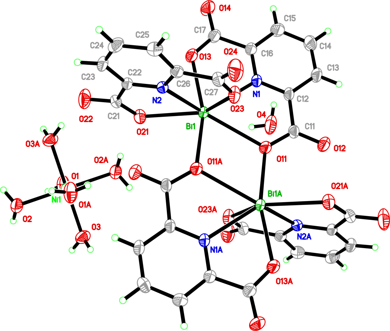
Fig. S1. The molecular structure of (II), showing the atom-labelling scheme. Displacement ellipsoids are shown at the 40% probability level. [Symmetry code: (A) -x+1, -y+1, -z+1 .]
