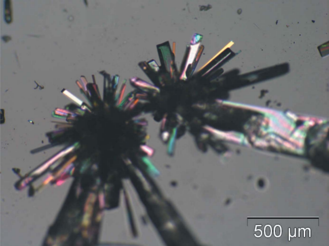
Fig. 4. Druses of codeine phosphate hemihydrate crystals grown by evaporation of a DMF solution.
