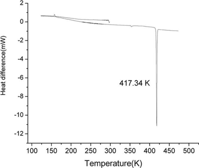
Fig. 3S. DSC plot for 1,1'-Bis-2,2'-naphthol biscarbonate (278 K/min) with the melting point at 417.34 K.
