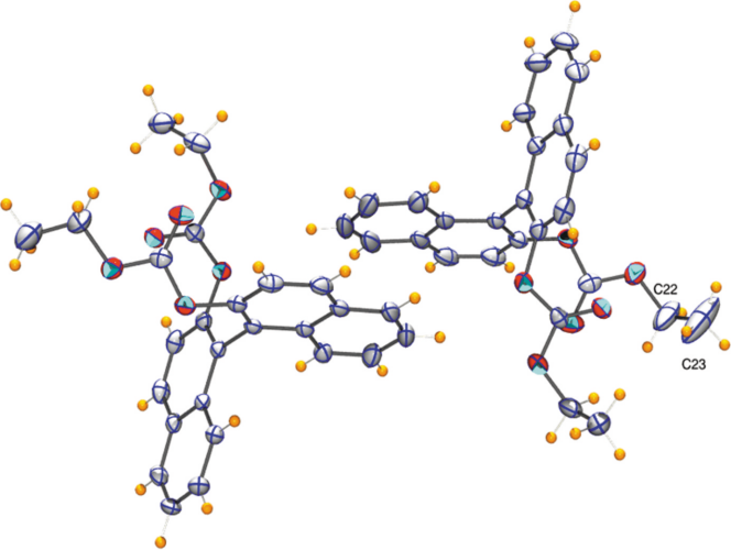
Fig. 2S. ORTEP diagram with 50% displacement ellipsoid probability at 150 K.
