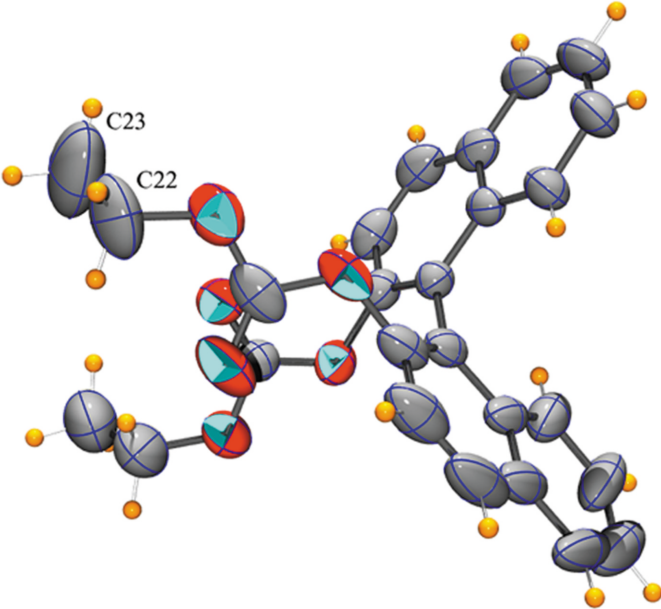
Fig. 1S. ORTEP diagram with 30% displacement ellipsoid probability at 393 K.
