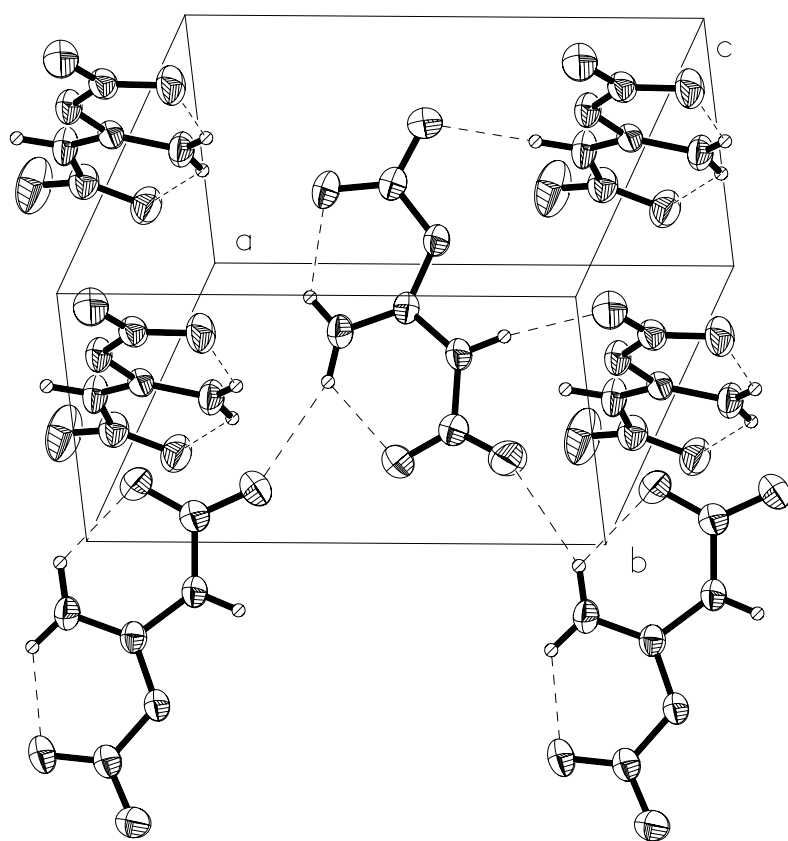
Supplementary Fig. 2. The packing arrangement in the crystal of (I). Dashed lines indicate intra- and intermolecular hydrogen bonds.
