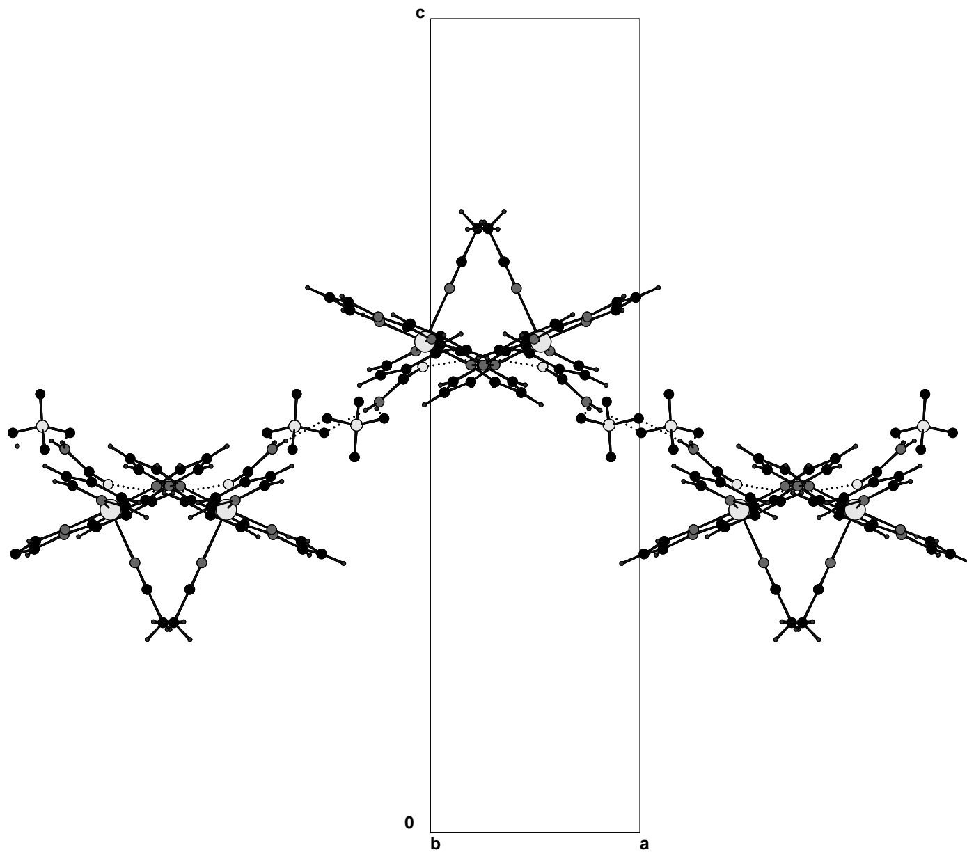
A projection of the structure of the title compound onto the (010) plane showing the zig-zag construction of the 2-D sheet (Cu, large pale grey spheres; C, intermediate black spheres; N, intermediate dark grey spheres; O, intermediate pale grey spheres; B, small pale grey spheres; F, intermediate black spheres).
